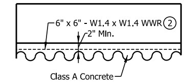
TYPICAL LONGITUDINAL SECTION
